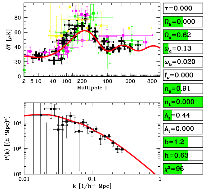
FIG. 10. The CMB and LSS power spectra for the “concordance” model from Table 1. Animated versions of this figure, where the effect of changing one parameter at a time can be viewed, are available at www.hep.upenn.edu/~max/concordance.html . The plotted model has bias b \approx 1.2 , redshift distortion parameter \beta = 0.47 and hubble parameter h = 0.63 .
