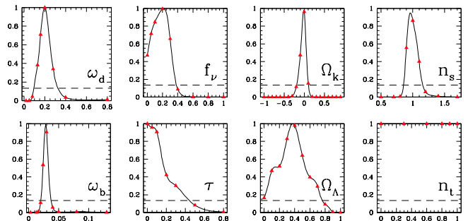
FIG. 3. Constraints on individual parameters using only CMB and LSS information. The quoted 95% confidence limits are where each curve drops below the dashed line.
