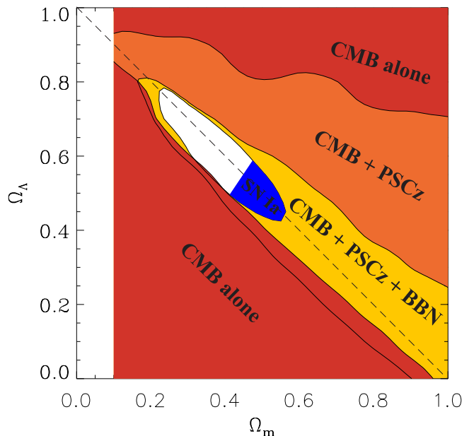
FIG. 5. Constraints in the (\Omega_m, \Omega_\Lambda) -plane. The shaded regions are ruled out at 95% confidence by the information indicated. The allowed (white) region is seen to be centered around flat models, which fall on the dashed line.
