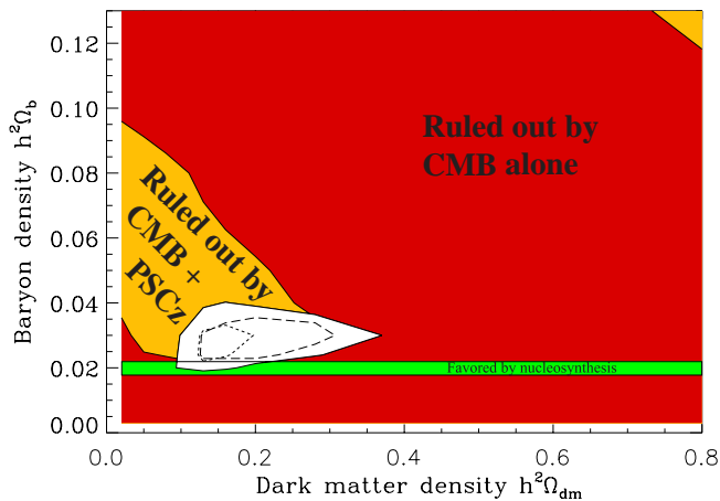
FIG. 7. Constraints in the (\omega_{dm}, \omega_b) -plane. As in the previous figure, adding PSCz prohibits high baryon solutions and allows slightly lower \omega_b -values than CMB alone. The dashed curve within the allowed (white) region show the sharper constraint obtained when imposing the priors for a flat, scalar scale-invariant model ( \Omega_k = r = 0, n_s = 1 ). The dotted curve shows the effect of requiring negligible neutrino density ( f_\nu \sim 0 ) in addition.
