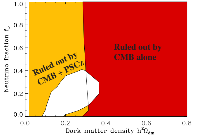
FIG. 8. Constraints in the (\omega_{dm}, f_\nu) -plane. The shape of the allowed (white) region explains why the prior f_\nu = 0 tightens the upper limit on the dark matter density. The vertical line shows the CMB-only boundary before PSCz is added.
