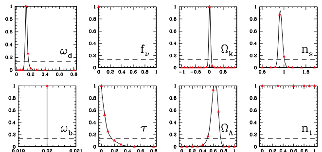
FIG. 4. Like the previous figure, but adding the “concordance” priors \omega_{\text{b}} = 0.02 , h = 0.74 \pm 0.08 and f_\nu \sim 10^{-3} .
